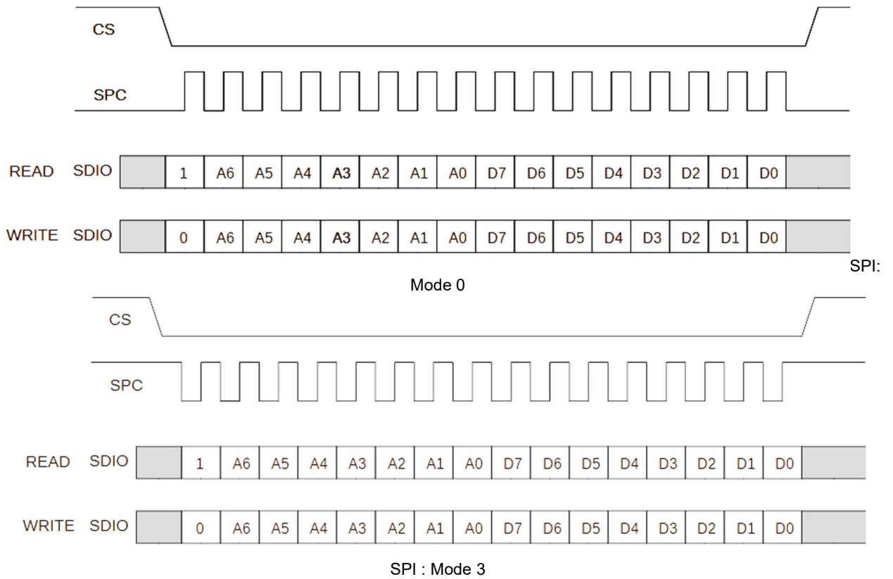
Figure 31. SPI 3-Wire Single Byte Read and Write Transactions
