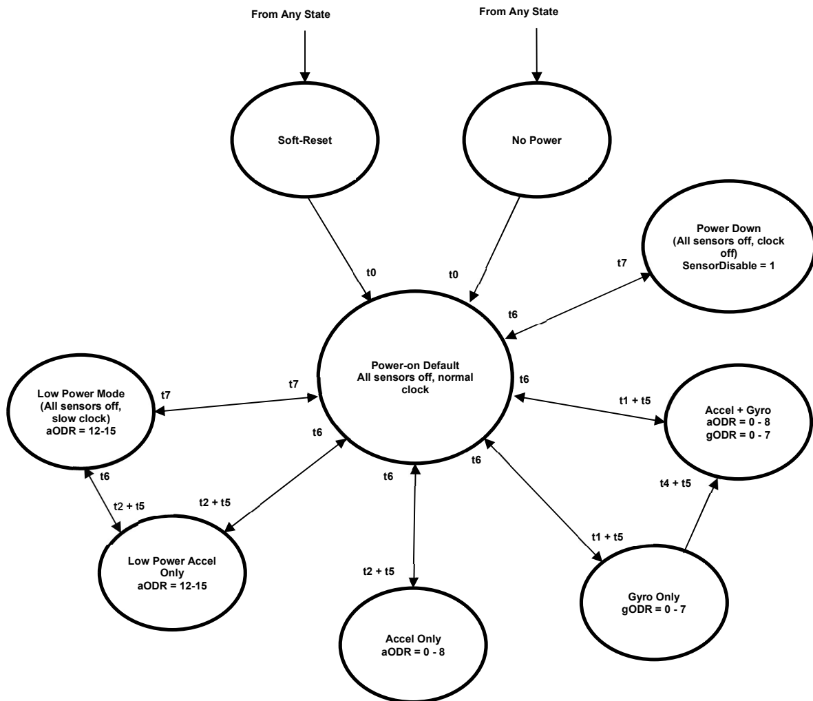
Figure 16. Operating Mode Transition Diagram
