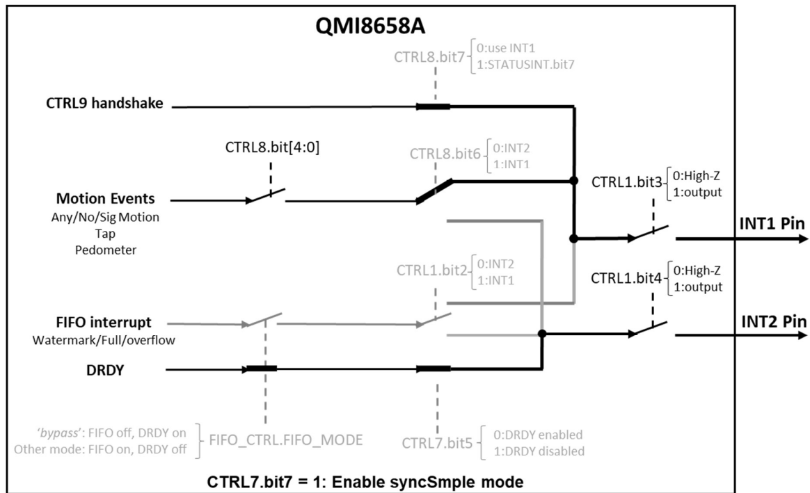
Figure 14. Interrupt Map of SyncSample Mode
