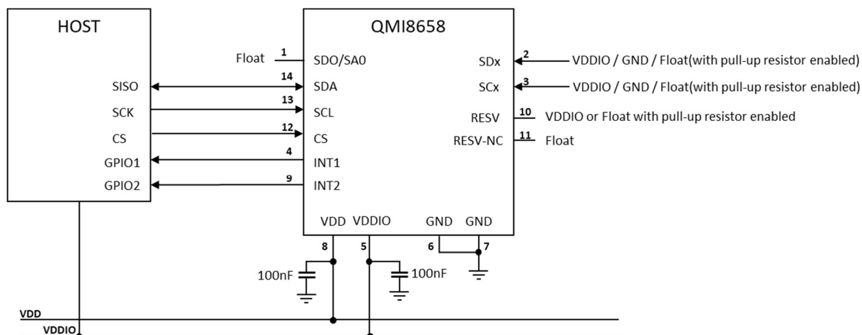
Figure 5. 3-Wire SPI-UI mode
