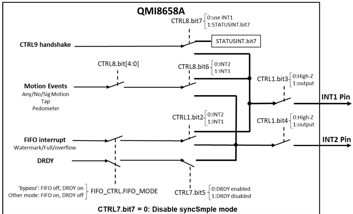
Figure 15. Interrupt Map of SyncSample Mode
