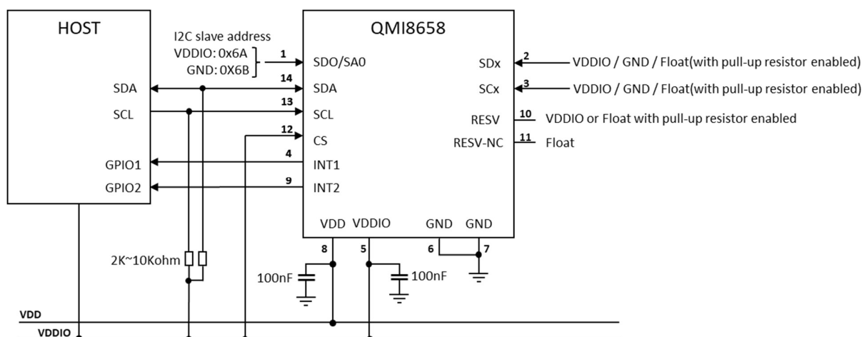
Figure 6. I3C/I2C-UI mode
