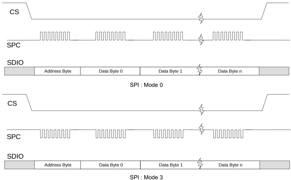
Figure 32. SPI 3-Wire Multi-Byte Read and Write Transactions
