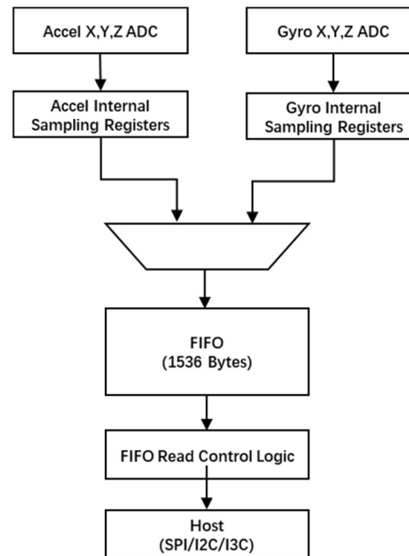
Figure 17. FIFO Data Flow
