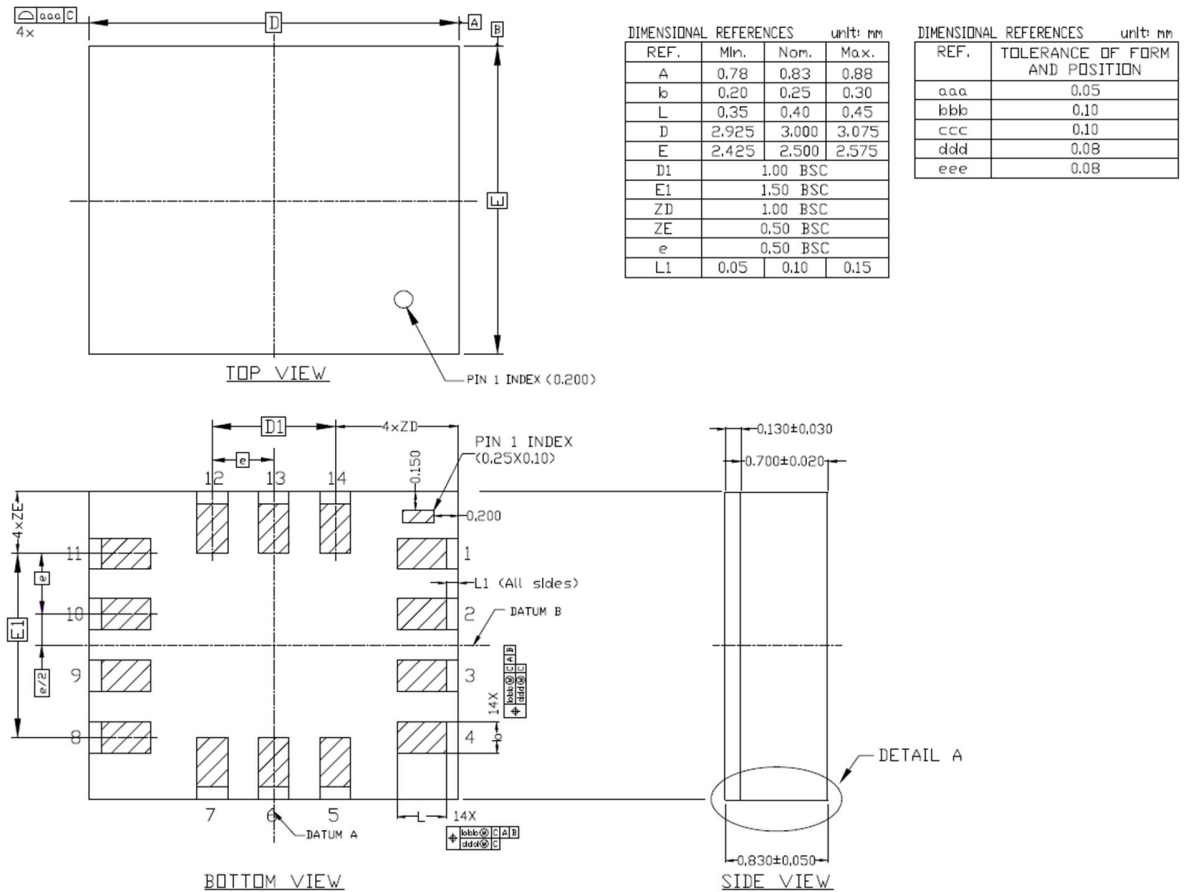
Figure 36. 14 Pin LGA 2.5 x 3.0 x 0.83 mm Package
