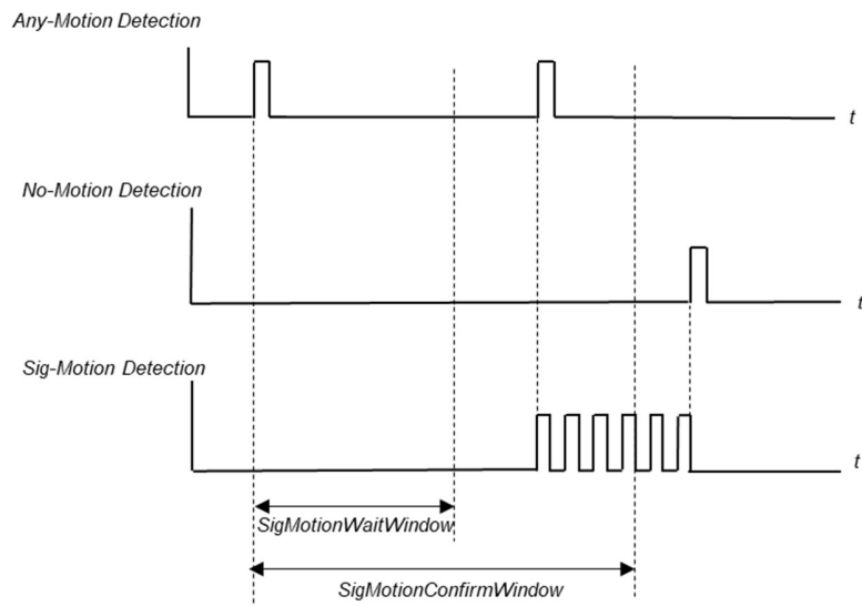
Figure 20. Significant-Motion interrupt detection
