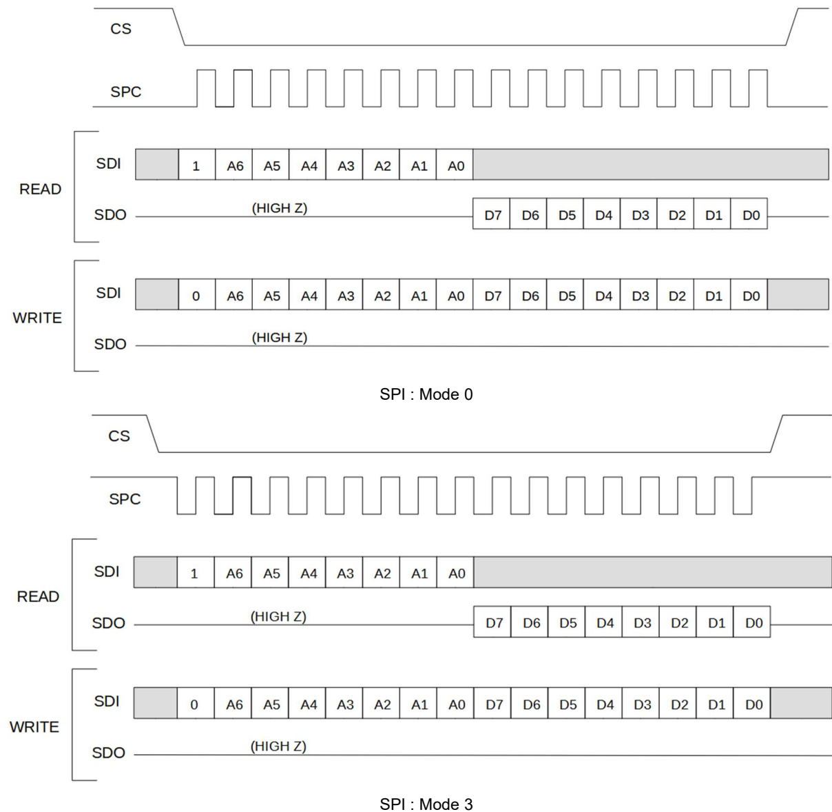
Figure 29. SPI 4-Wire Single Byte Read and Write (Mode 0 and Mode 3)
