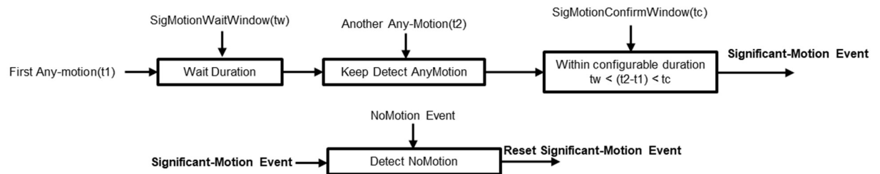
Figure 23. Significant-Motion Detection Flow
